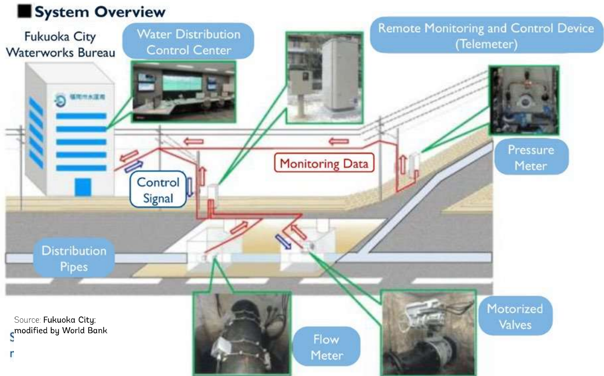
FIGURE 2.2 Overview of Water Distribution Control Center
