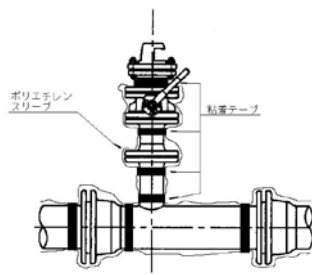
(市型消火栓)
